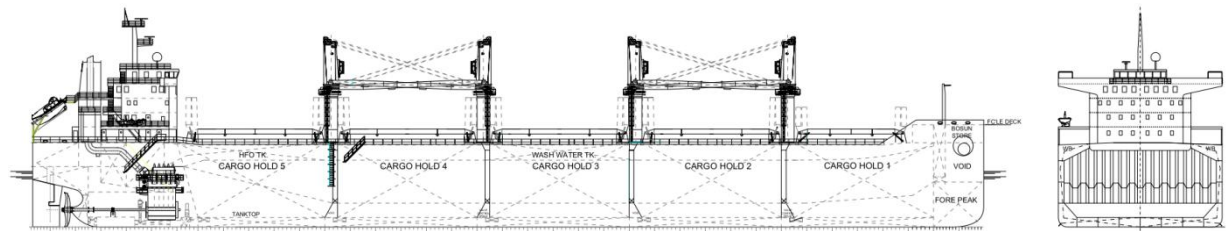
SD41, Efficient 41,000 DWT bulk carrier design by Foreship BlueTech Ltd.
